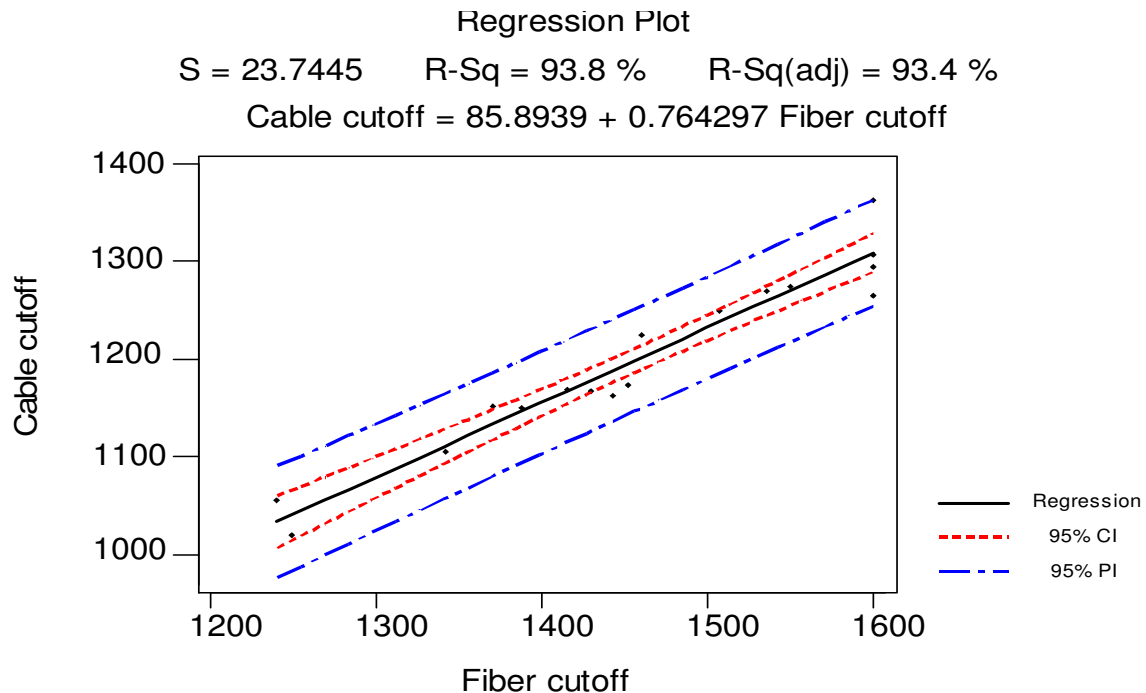
Figure 3 Regression plot between Fiber and Cable Cut-off Wavelength (G655, DOF-LITE™ LEA)
