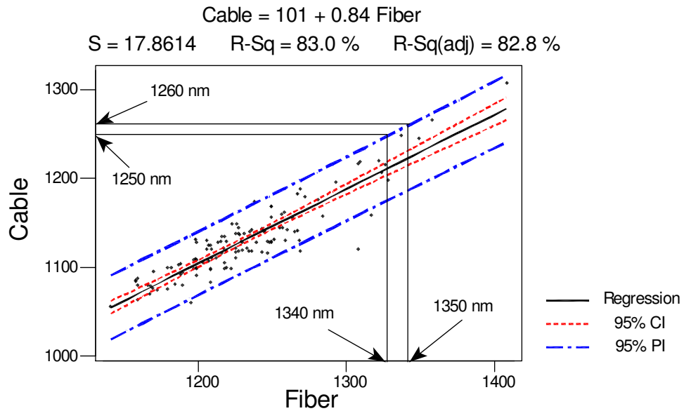
Figure 1 Regression plot between Fiber and Cable Cut-off Wavelength (SMF dispersion unshifted fiber, G652)
