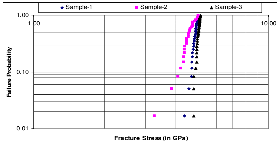
Figure 8 Weibull probability plot of tensile strength values at day 180
