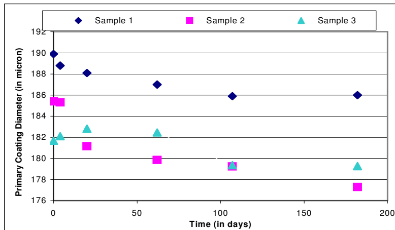
Figure 1 Change in primary coating diameter with time aging after fiber drawing
