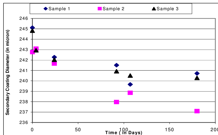
Figure 2 Change in secondary coating diameter with time aging after fiber drawing
