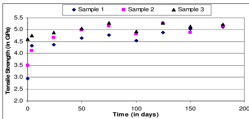
Figure 5 Change in tensile strength with time aging after fiber drawing
