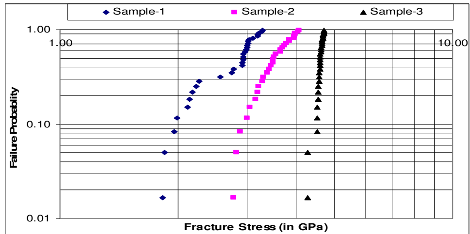
Figure 7 Weibull probability plot of tensile strength values at day 0
